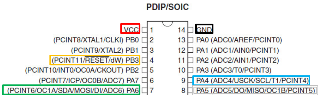
Figure 1-1. Pinout ATtiny24/44/84
