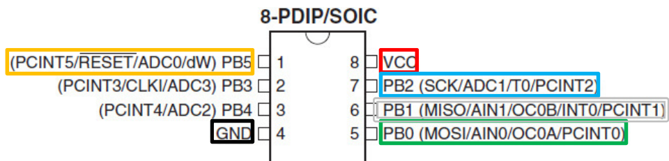
Figure 1-1. Pinout ATtiny13/ATtiny13V
