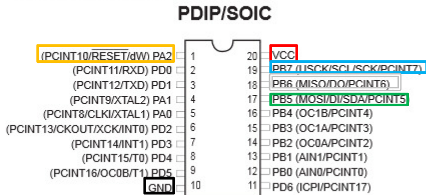
Figure 1-1. Pinout ATtiny2313A/4313
